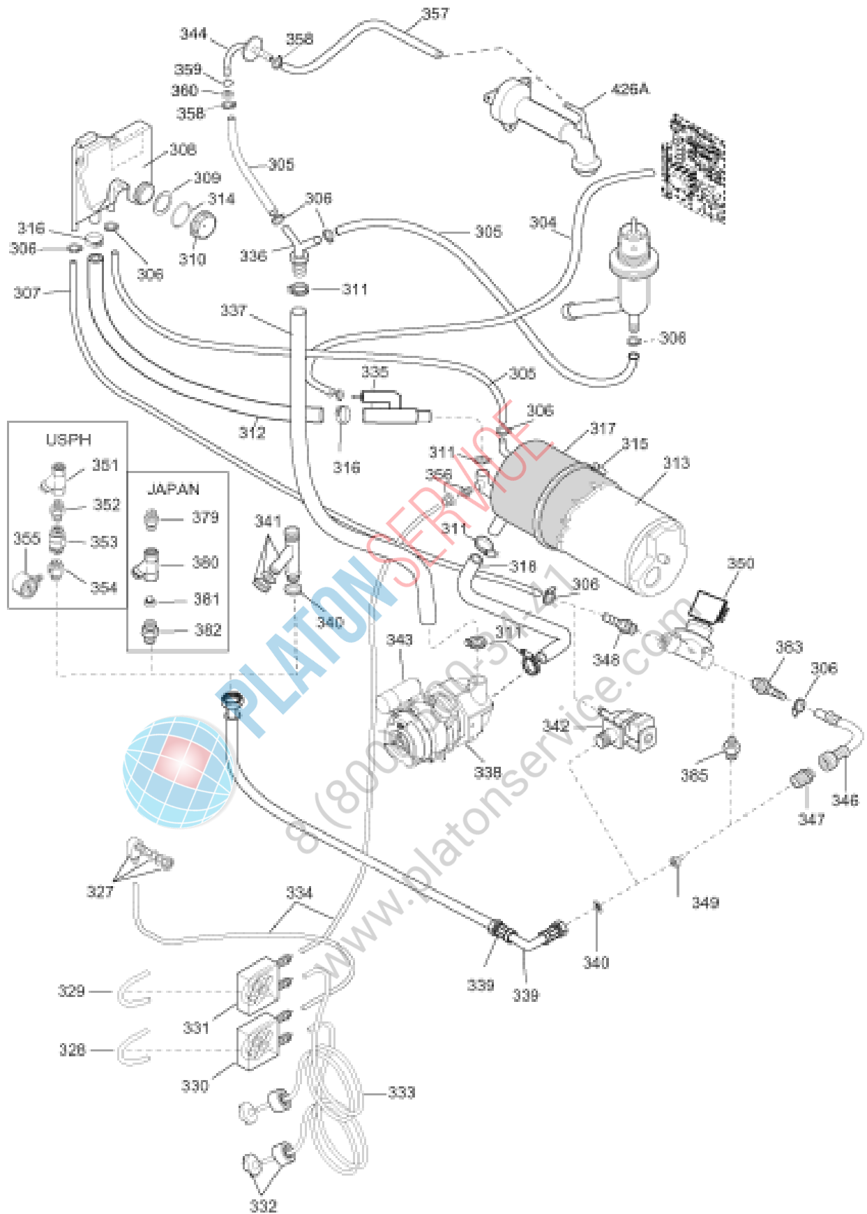
III 641804p3 Circuiti idraulico / Hydraulic circuit
